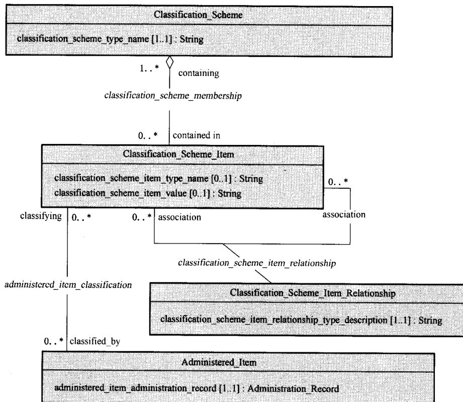
Figure 7—Classification metamodel region
