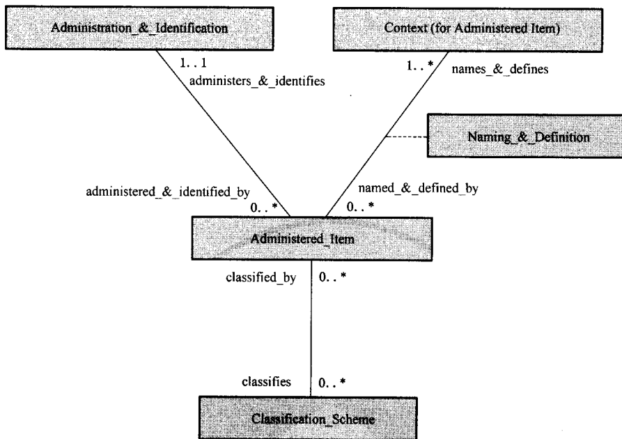
Figure 1—Common facilities for all Administered Items
