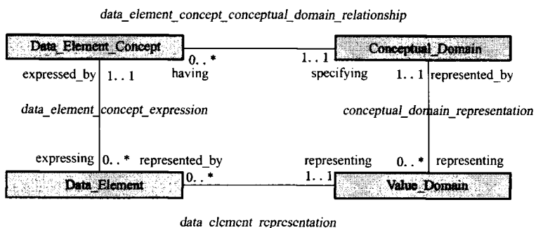
Figure 3—High-level metamodel
