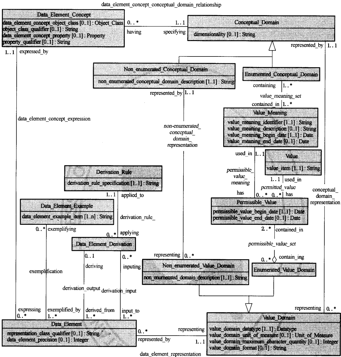
Figure 11—Consolidated metamodel
