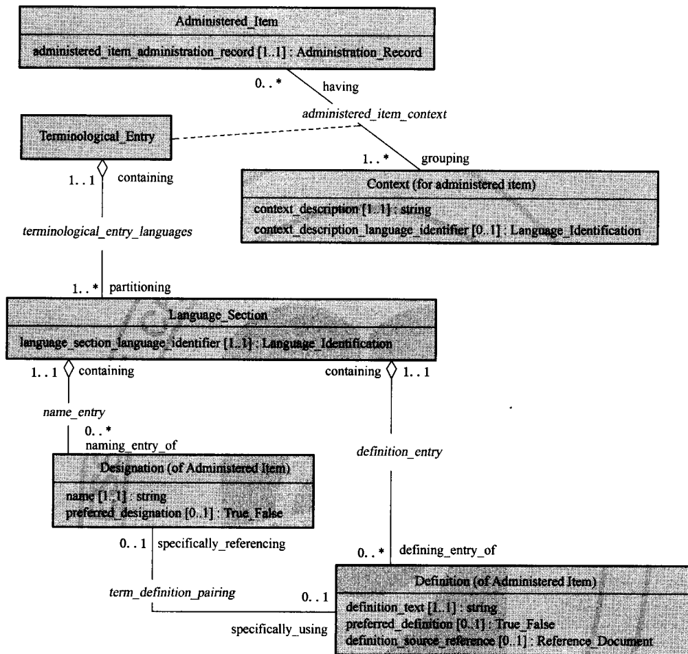
Figure 6—Naming and Definition metamodel region
