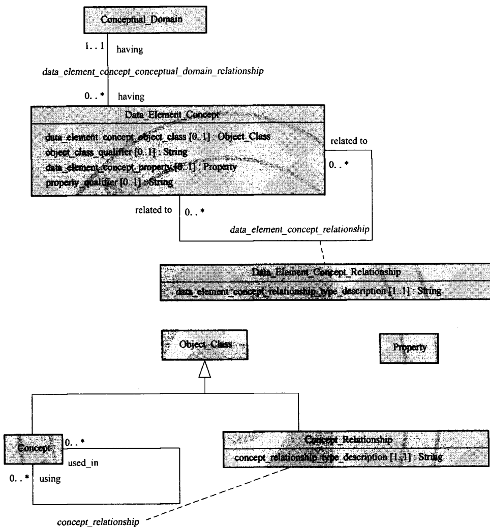
Figure 8—Data Element Concept metamodel region
