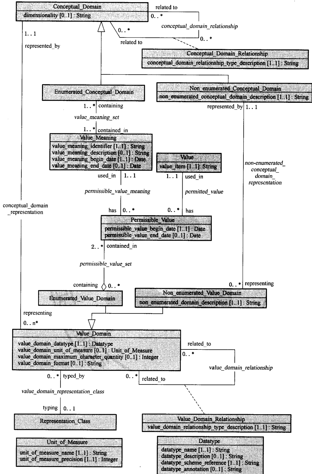
Figure 9—Conceptual and value domain metamodel region
